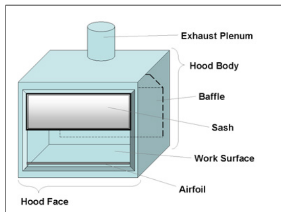
Figure IV-III. Fume Hood
